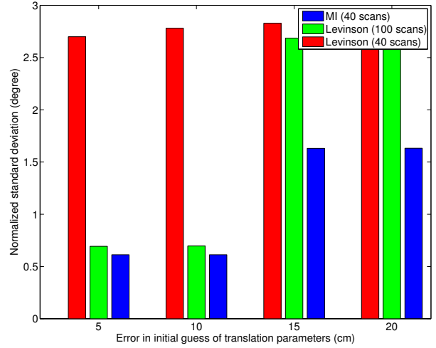
(d) Standard deviation of estimated rotation when error in initial guess of rotation parameters is 10° and error in translation parameters is changed from 5 cm to 20 cm
