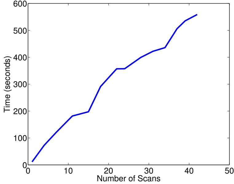
Figure 13: Computation time as a function of the number of scans used for calibration. Computation time increases as the number of data points are increased (1 scan contains approximately 80,000–100,000 3D points). More data results in better calibration performance, so there is a trade-off between computation time and the robustness of the algorithm.
