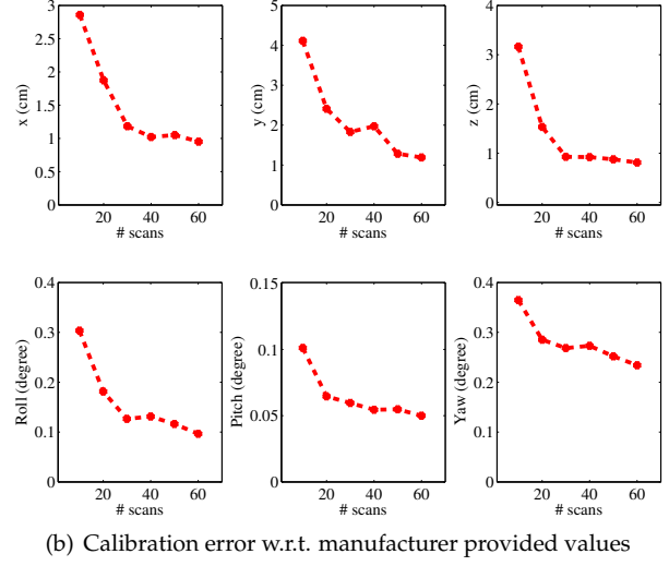
Figure 16: Comparison with manufacturer ground-truth. (a) A depiction of the coordinate frames corresponding to each camera ( c_i ) and camera head ( H ) of the Ladybug3 omnidirectional camera system. (b) Plotted are the mean absolute error in the relative-pose calibration parameters for the two side looking cameras ( c_2 and c_5 ), i.e. |\mathbf{X}_{c_2c_5} - \hat{\mathbf{X}}_{c_2c_5}| , versus the number of scans used to estimate these parameters. The mean is calculated over 100 trials of sampling N scans per trial \{N = 10, 20, \dots, 60\} . We see that the error decreases as the number of scans are increased.
