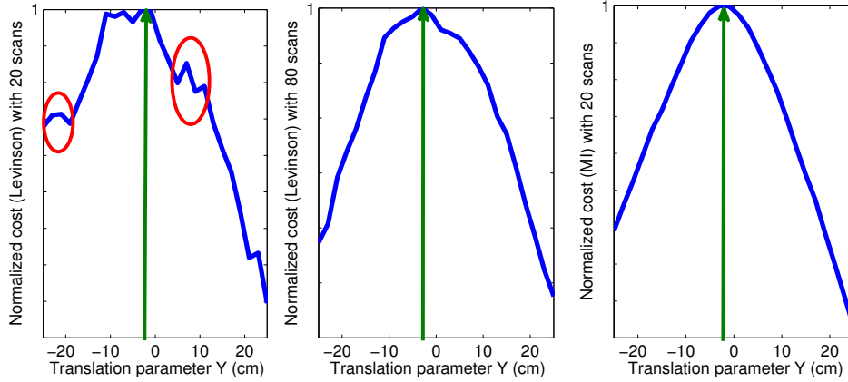
(b) Normalized cost for Levinson with 20, Levinson with 80, and MI-based with 20 scans
