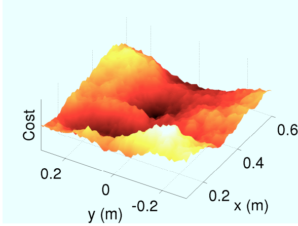
(c) Cost function with 1 scan
