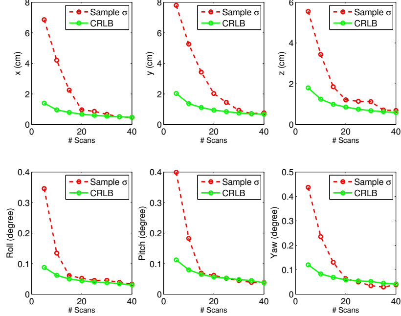
Figure 11: 3D laser and omnidirectional camera multi-view calibration results. Here we use all five horizontal images from the Ladybug3 omnidirectional camera during the calibration. Plotted is the uncertainty of the recovered calibration parameters versus the number of scans used. The red (dashed line) plot shows the sample-based standard deviation ( \sigma ) of the estimated calibration parameters calculated over 1000 trials. The green (solid line) plot represents the corresponding CRLB of the standard deviation of the estimated parameters. Each point on the abscissa corresponds to the number of aggregated scans used per trial.
