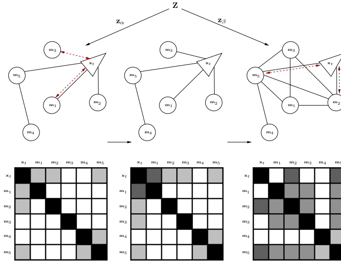
Fig. 2. Sparsification as performed by ESEIFs during the measurement update step. At time t , three of the mapped features are active, \mathbf{m}^a = \{\mathbf{m}_1, \mathbf{m}_2, \mathbf{m}_5\} and two are passive, \mathbf{m}^- = \{\mathbf{m}_3, \mathbf{m}_4\} as indicated by shaded off-diagonal elements of the information matrix. The robot makes three observations of active features, \mathbf{z}_1 , \mathbf{z}_2 , and \mathbf{z}_5 , and one of a passive feature, \mathbf{z}_3 . The first step of the ESEIF sparsification algorithm, as shown in the left-most diagram, is to update the posterior based upon a subset of the measurements, \mathbf{z}_\alpha = \{\mathbf{z}_1, \mathbf{z}_3\} , resulting in a stronger constraint with \mathbf{m}_1 as well as the formation of a link with \mathbf{m}_3 , as depicted in the middle figure. Sparsification then proceeds with the marginalization of the vehicle pose and subsequent relocation of the robot based upon the remaining measurements, \mathbf{z}_\beta . The implication on the information matrix is the connectivity of the initial set of active features and a desired restriction on the number of constraints with the vehicle pose.
