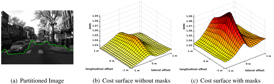
Figure 5: Sample of improvement of the NMI cost surface when obstacle masks are used.
